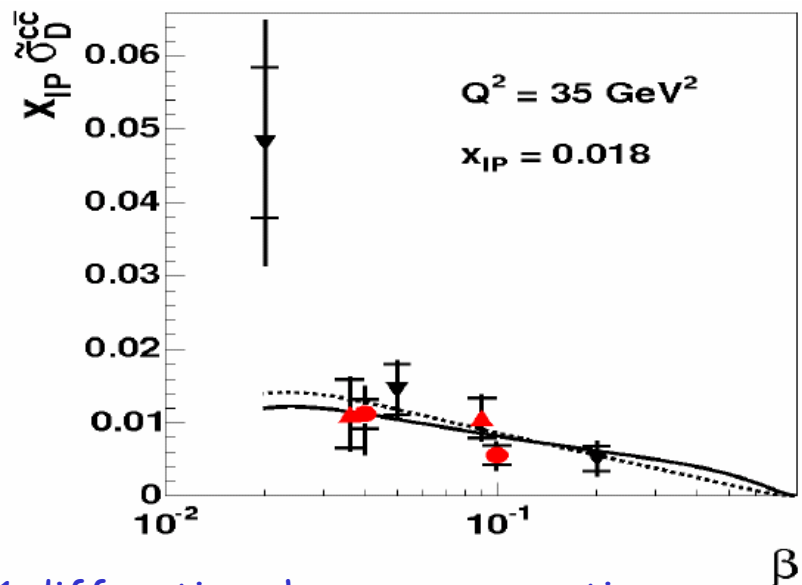
H1 diffractive charm cross sections compared to predictions using H1-DPDFs
