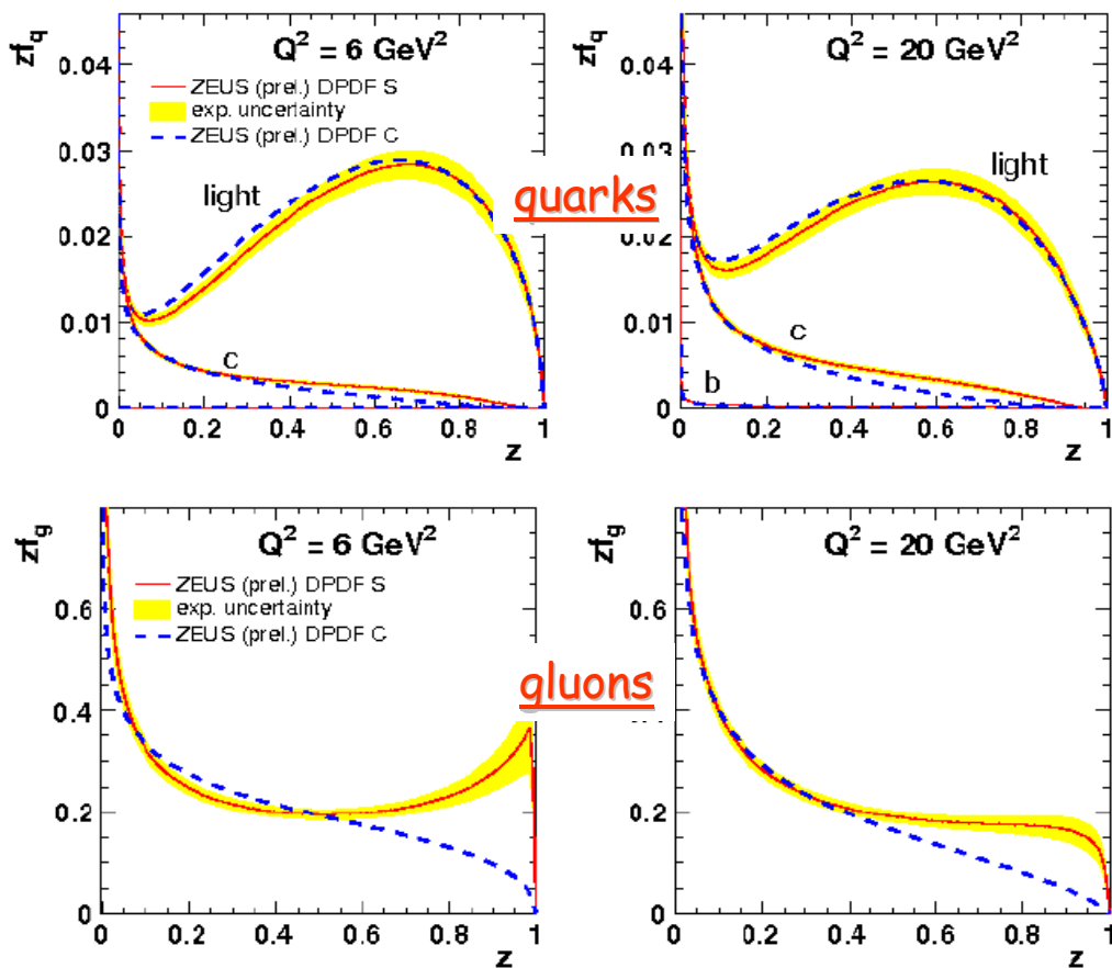
ZEUS fit S vs fit C
