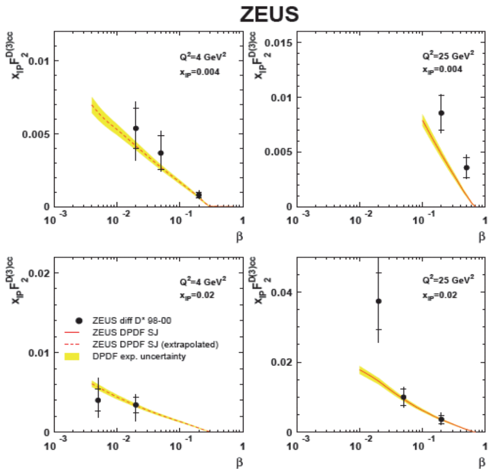
ZEUS DPDF fit SJ predictions compared to charm diffractive structure function x_{IP} F_2^{D(3)cc}
