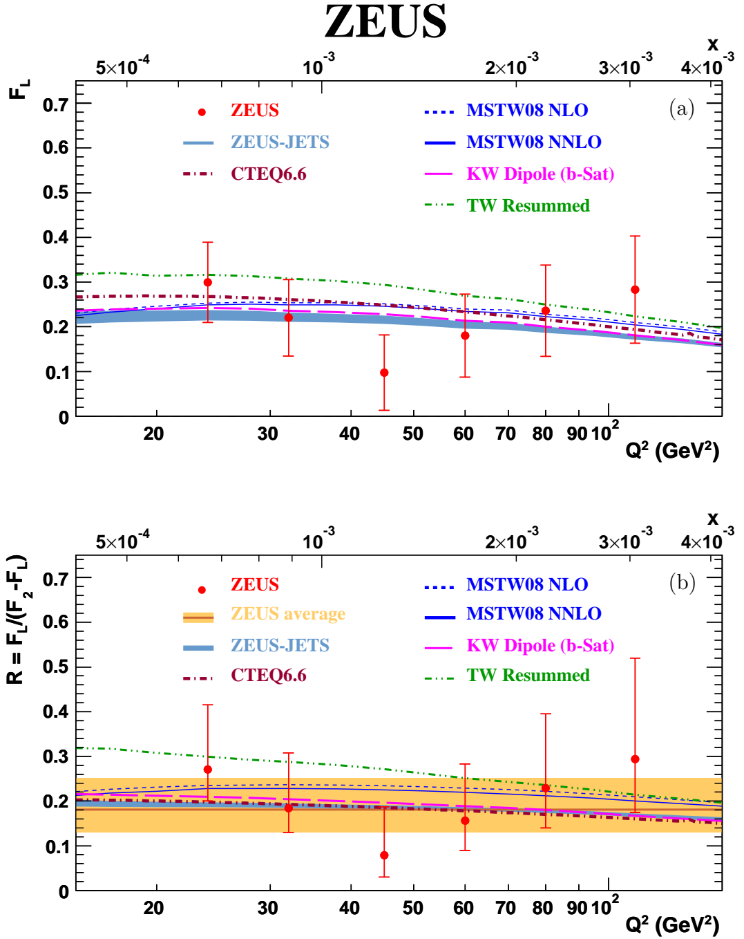
Figure 4: Values of (a) F_L and (b) R as a function of Q^2 . The error bars on the data represent the combined statistical and systematic uncertainties. A further \pm 2.5\% correlated normalisation uncertainty is not included. The shaded band labelled ZEUS average represents the 68% probability interval for the overall R . The lines represent various model predictions (see text for details).
