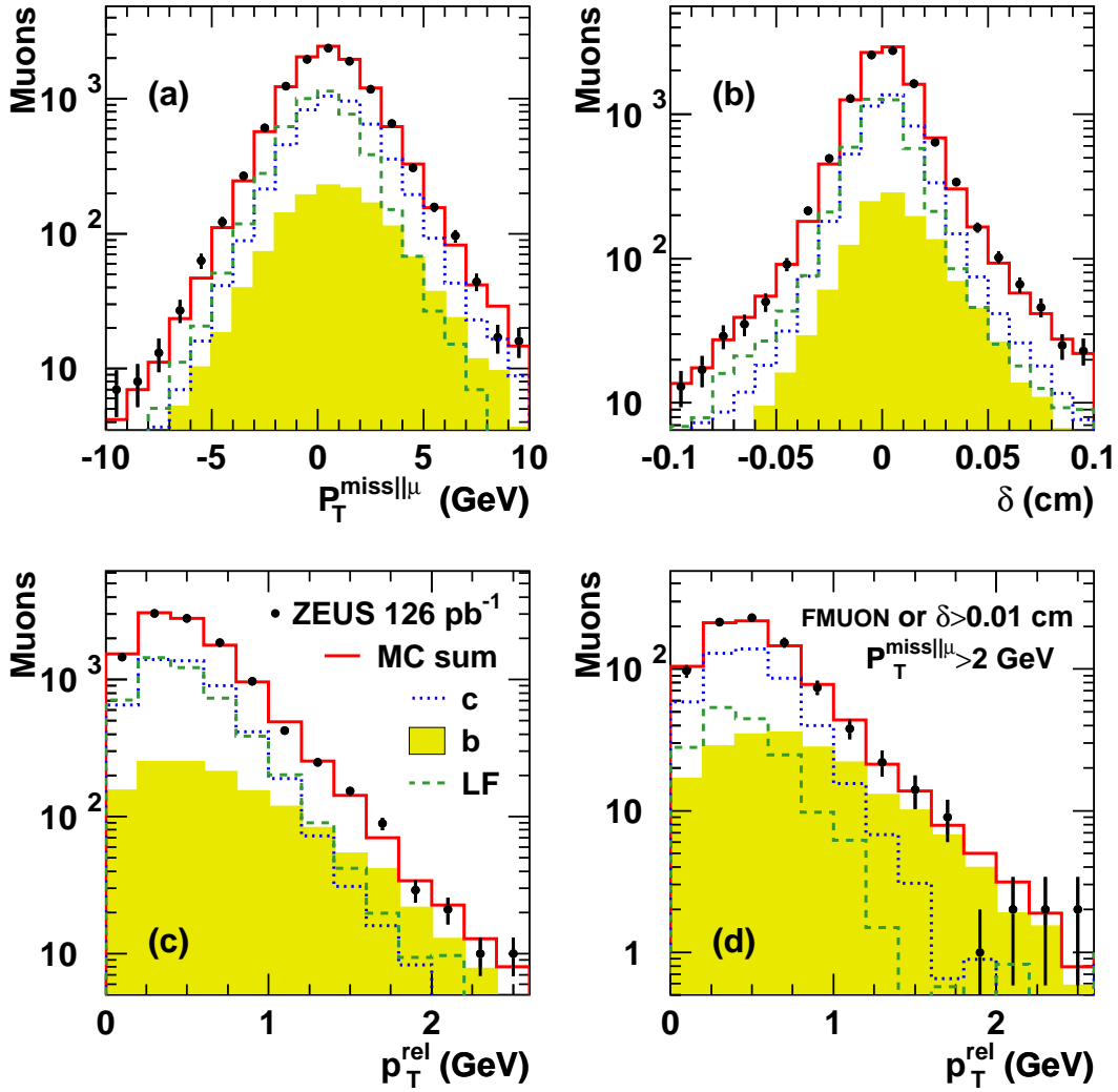
Figure 1: Distributions of (a) p_T^{\text{miss}||\mu} , (b) \delta , (c) p_T^{\text{rel}} for the selected sample of muons in DIS, and of (d) p_T^{\text{rel}} for a signal-enriched subsample with p_T^{\text{miss}||\mu} > 2 GeV and either a muon in FMUON or \delta > 0.01 cm. The data (points) are compared to the MC expectation (solid line) with the normalisation of the c (dotted line), b (shaded histogram) and light flavours (dashed line), LF, components obtained from the global fit. The error bars correspond to the square root of the number of entries.
