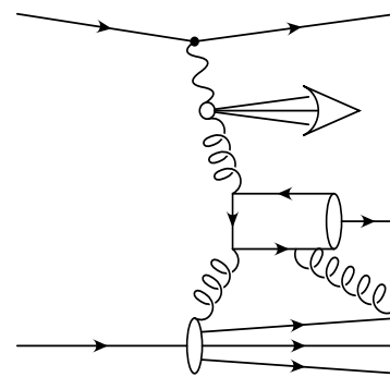
Resolved \gamma process
