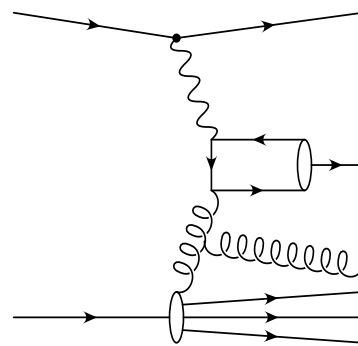
Direct \gamma processes
